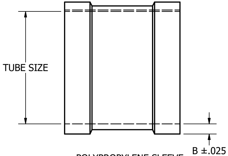
POLYPROPYLENE SLEEVE (TO FIT TUBING SIZE)
