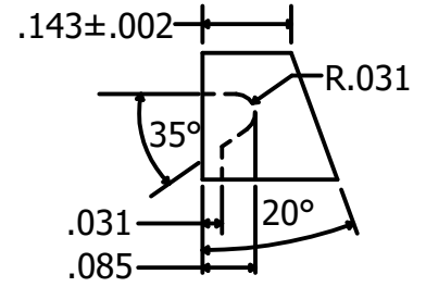
14WMP-1/2" GASKET GROOVE DETAIL
