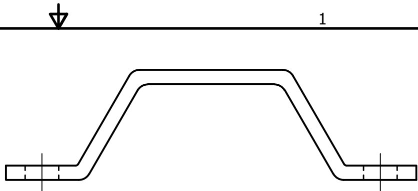
BRACKET (2-REQUIRED)
