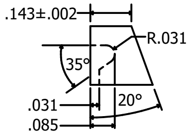
Gasket Groove Detail 1/2" & 3/4" Sizes
