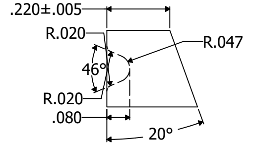
Gasket Groove Detail 6" to 12" * = .080 for 8" to 12"
